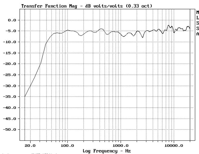
Amplitudenfrequenzgang (212T, 152Atue)
