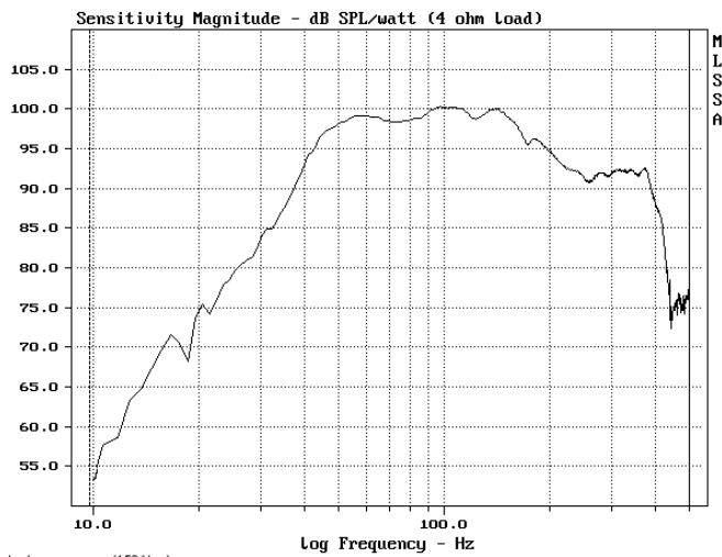
Amplitudenfrequenzgang (152Atue)
