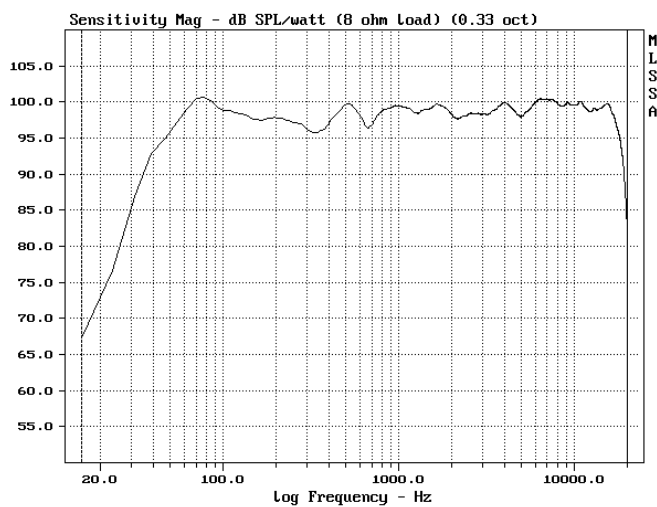
Frequency response GAE PS 4464T - PS 4464L
