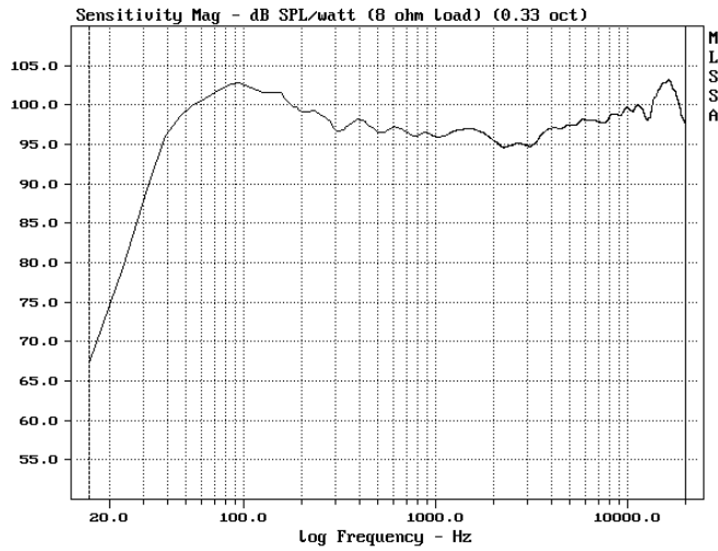
Frequency response
