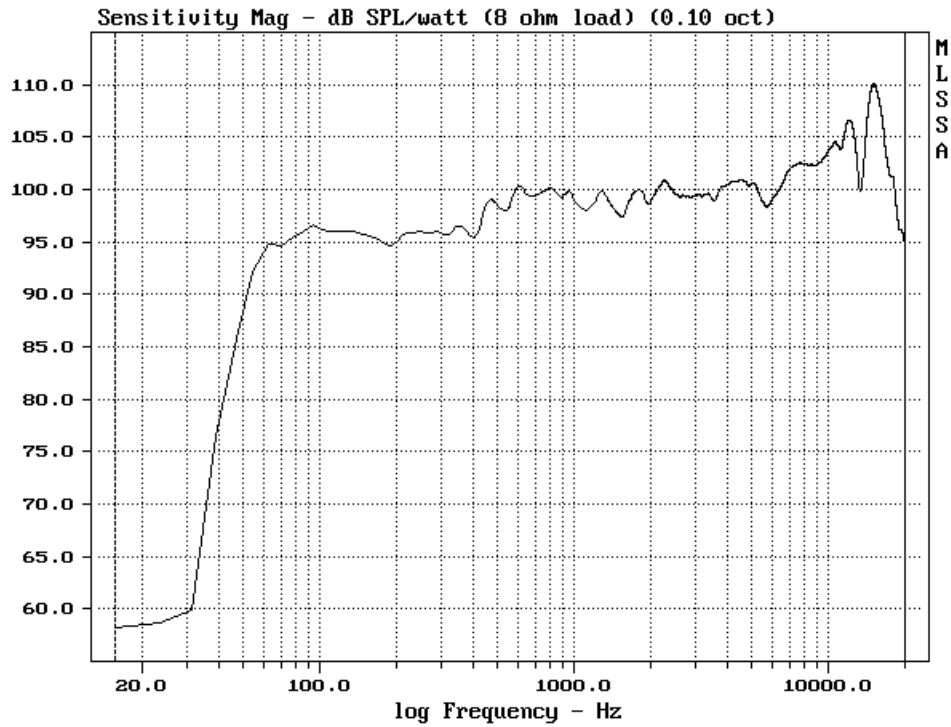
System 15-6 passiv Frequenzgang / Frequency Responce
