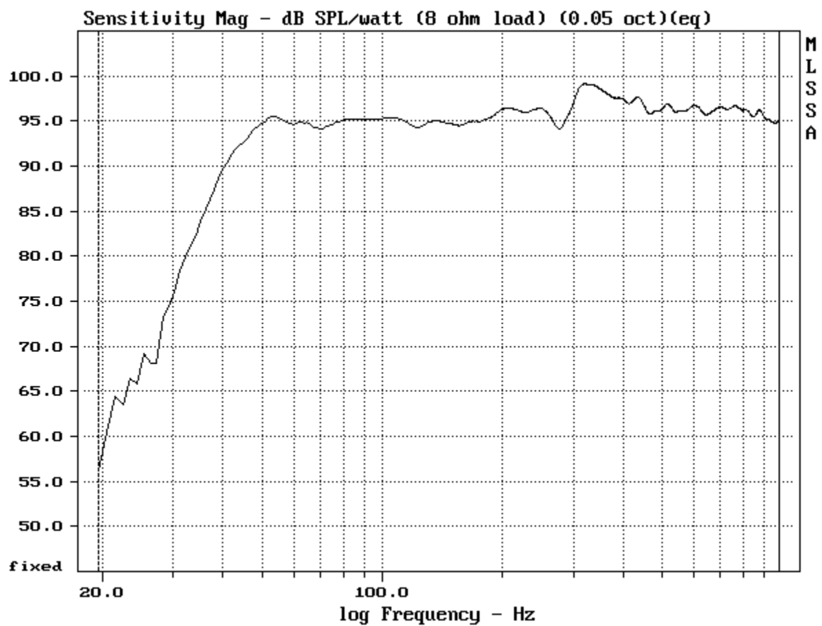
GAE BR15N Frequenzverlauf / Frequency Response
